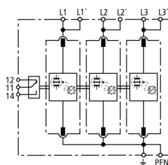
Basic circuit diagram DV M TNC 255 FM
