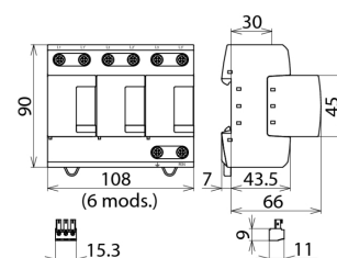
Dimension drawing DV M TNC 255 FM
